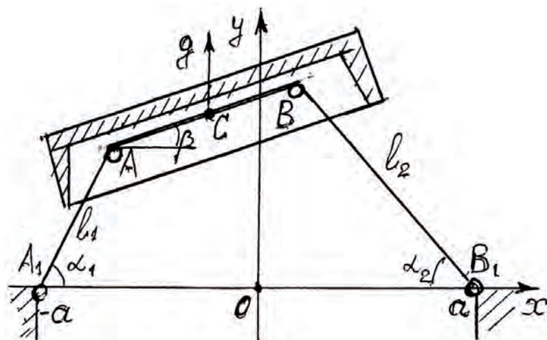
The measurement of some parameters of double-axis carriage movement on the weightless and stretchless rope is presented in this article.
